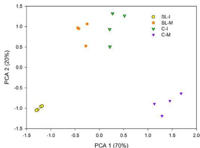
Fig. 5. Principal component analysis performed on the abundance of different soil N cycling genes studied ( nifH , nirS , nirK , nosZ , amoA -Arch and amoA -B) and 16S rRNA gene. SL-I: soil under salvage logging treatment sieved at 2 mm; SL-M: soil under salvage logging treatment sieved between 63 and 250 µm; C-I: control soil with tree retention sieved at 2 mm; C-M: control soil with tree retention sieved between 63 and 250 µm. Different letters above the bars indicate significant differences.
